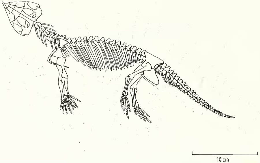
TEXT-FIG. 2. Restoration of the skeleton of Scaphonyx fischeri (MCZ 1664) lying in the position in which it was fossilized.
